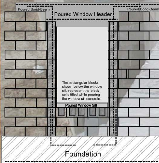
Cross sectional window detail
